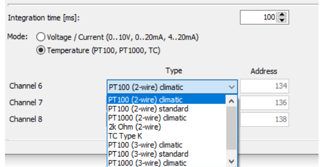
Configuration block addresses (in bytes) and measuring range configuration Analog Input in the ConfigStage Mode temperature
